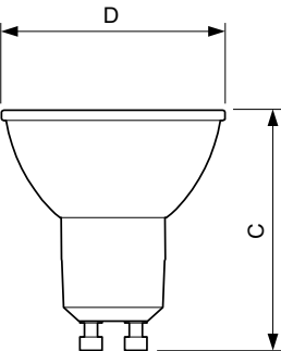
GU10 230V 4W-35W 260lm 100D 2700K GU10ND
