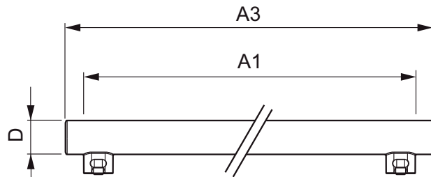
LEDtube S14S
